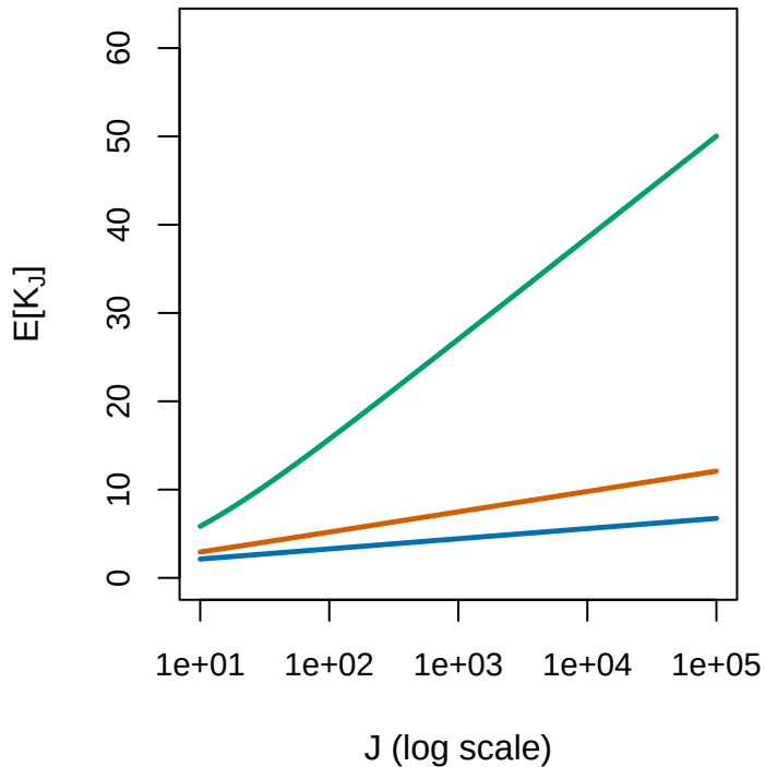
Logarithmic growth
