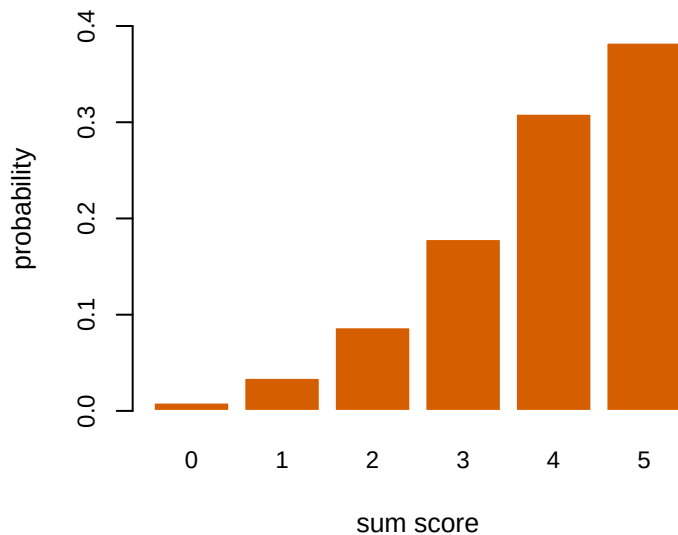
6 spread items: TV from normal G = 0.035
