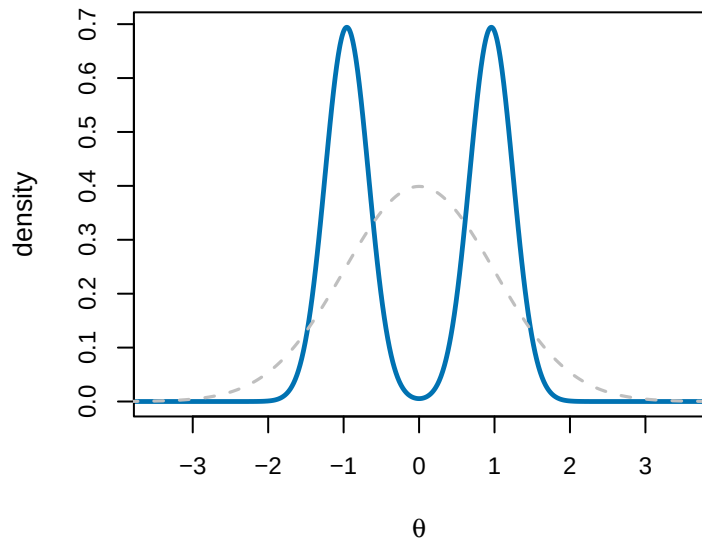
G is sharply bimodal
