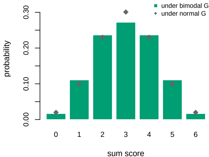
6 spread items: TV from normal G = 0.035
