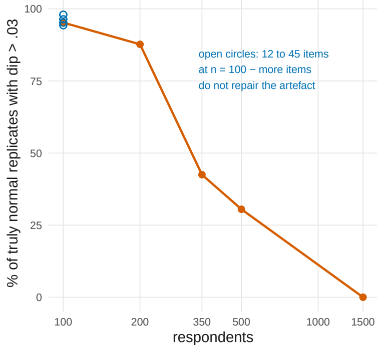
Spurious multimodality under a truly normal latent trait
