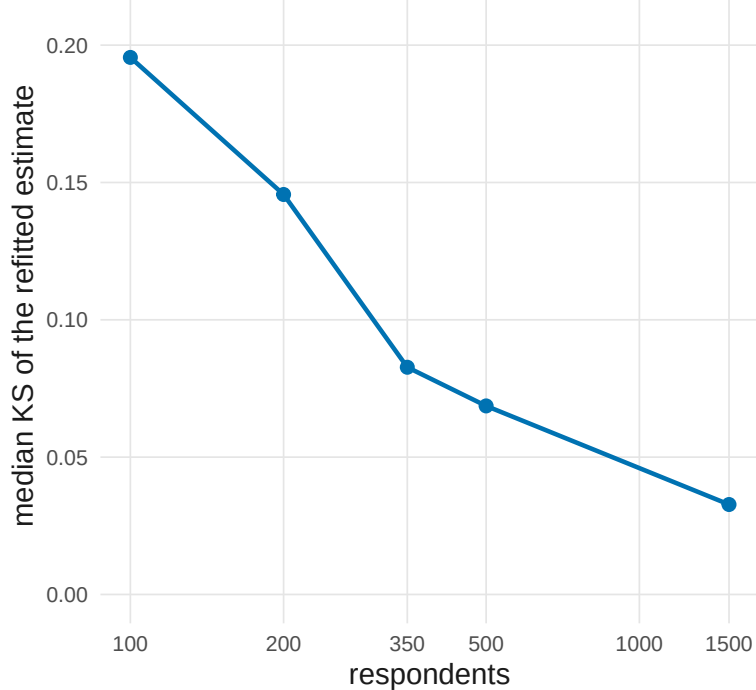
The estimation noise floor falls only with respondents
