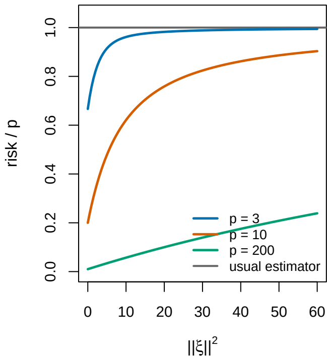
James–Stein risk, relative to p
