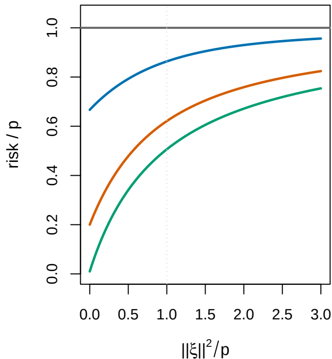
Against spread per coordinate
