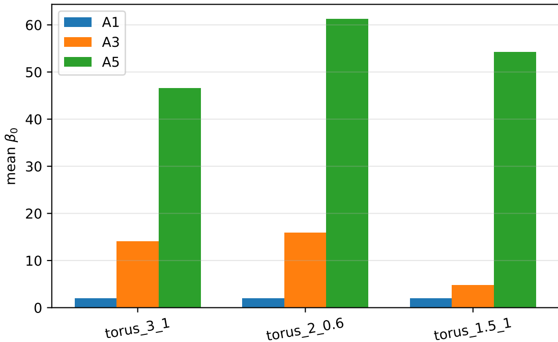
E4: genus 1, three embedded metrics
