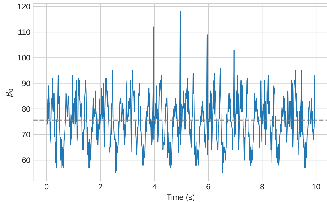
A7 / sphere_genus0 ( \sigma(\beta_0) = 11.0 )
