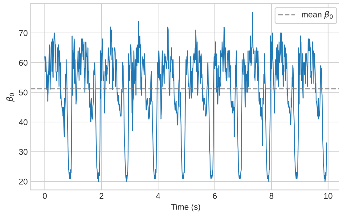
A7 / torus_genus1 ( \sigma(\beta_0) = 4.5 )
