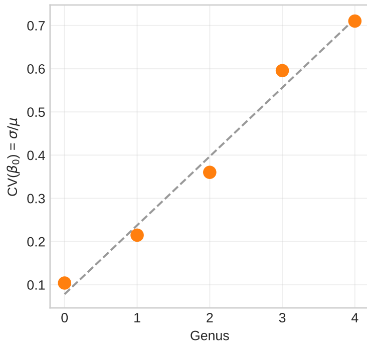
A3 (piano) — temporal variance of \beta_0 vs genus
