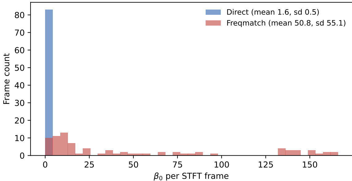
Sphere \times A3: per-frame \beta_0 distribution
