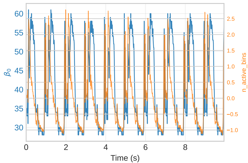
A7 — sphere (Spearman \rho = 0.838 )
