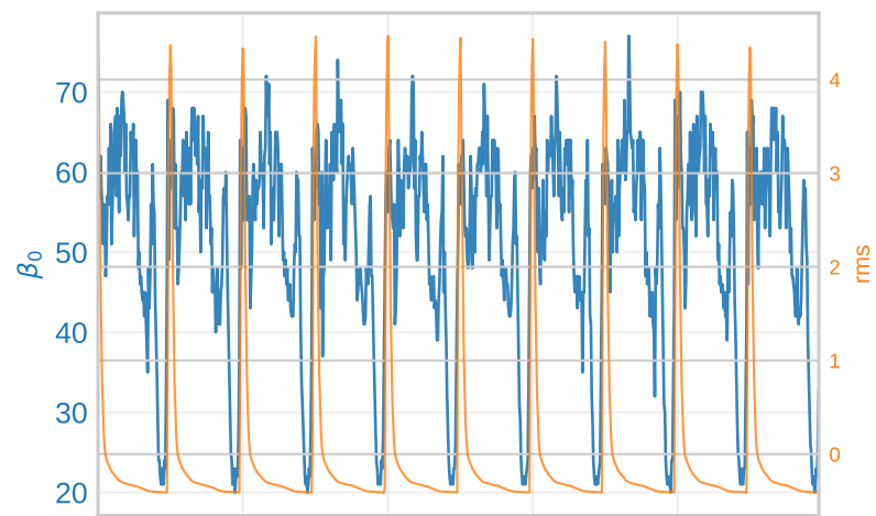
A3 — torus (Spearman \rho = 0.652 )
