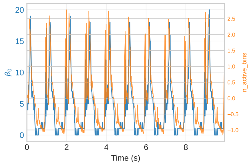
A7 — torus (Spearman \rho = 0.829 )
