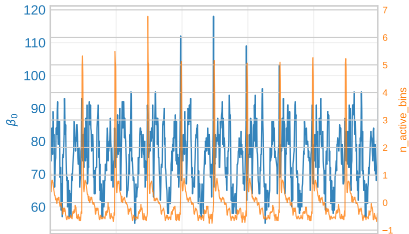
A3 — sphere (Spearman \rho = 0.451 )
