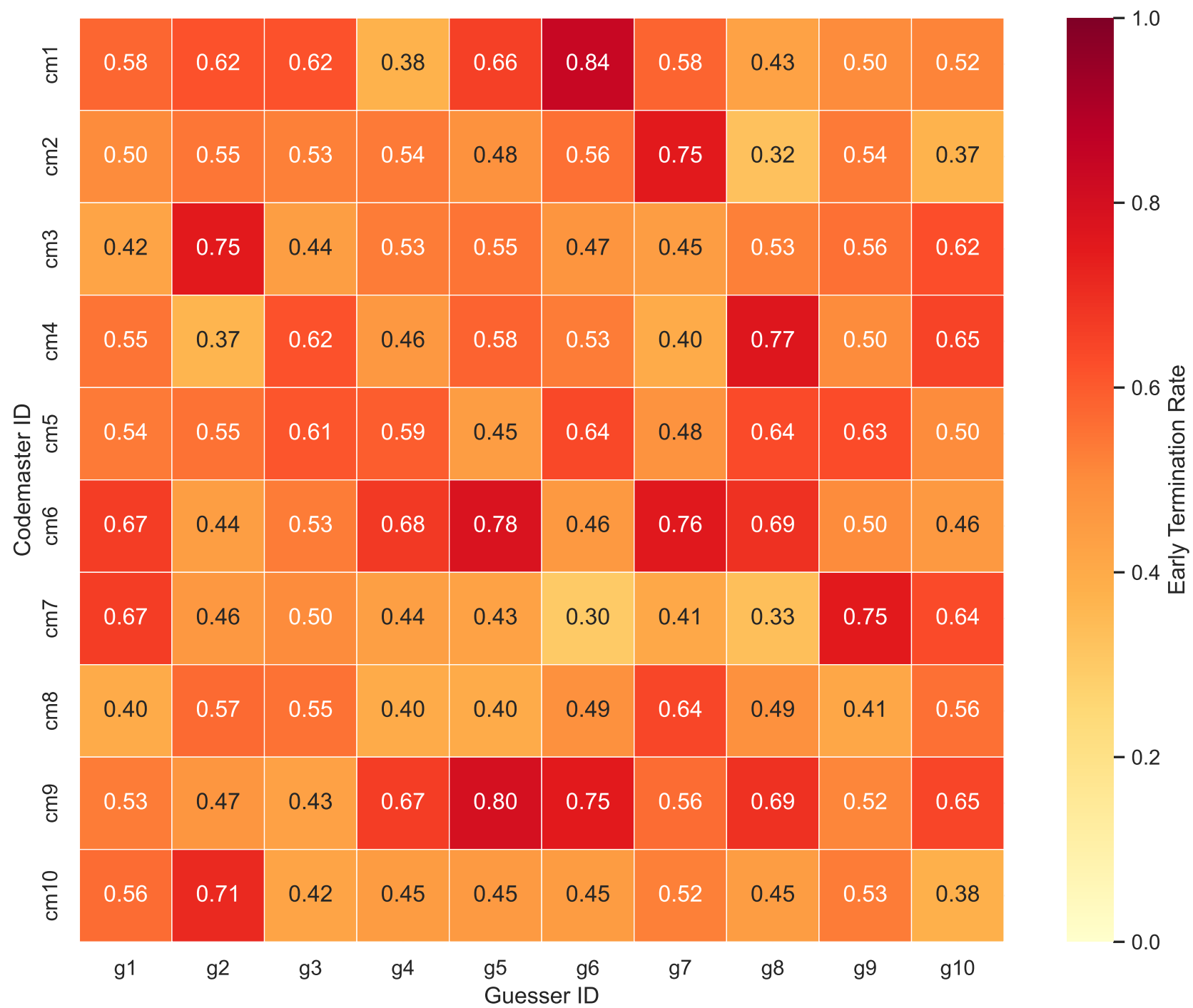
Early Termination Rate by Persona Pair
