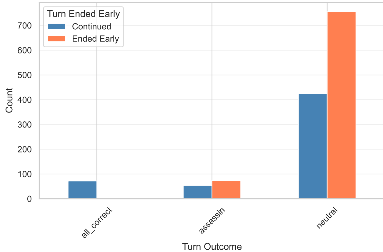
Early Termination by Turn Outcome
