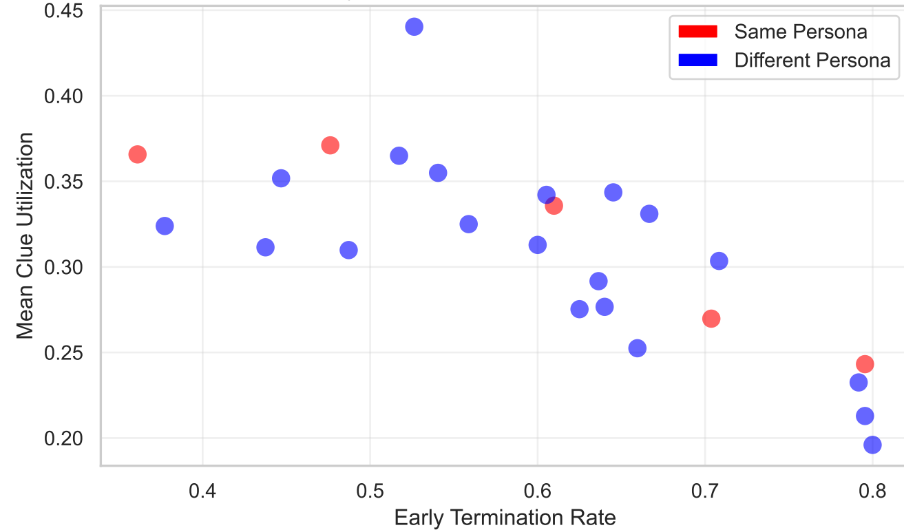
Early Termination vs Clue Utilization
