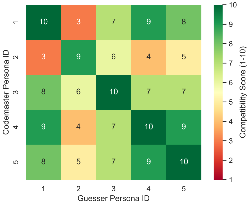
LLM-as-a-Judge Compatibility Matrix (Theory of Mind / Synergy)
