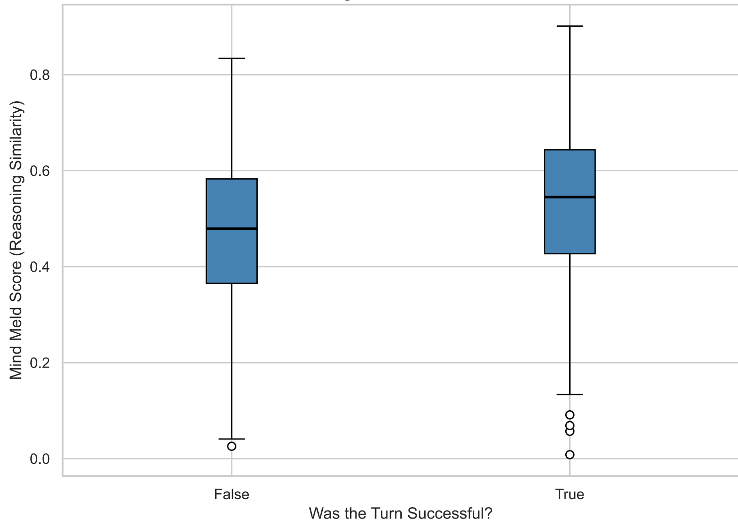
Does Semantic Alignment Correlate with Success?
