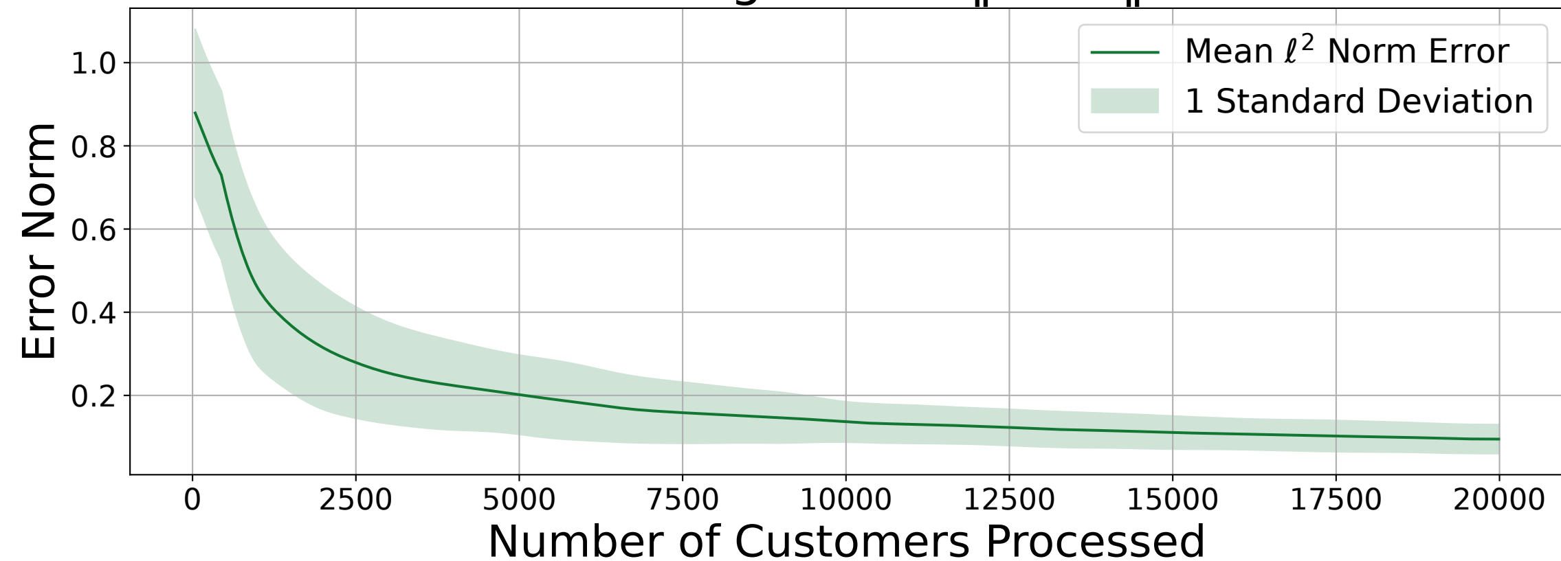
Convergence of \|\hat{\theta} - \theta\|
