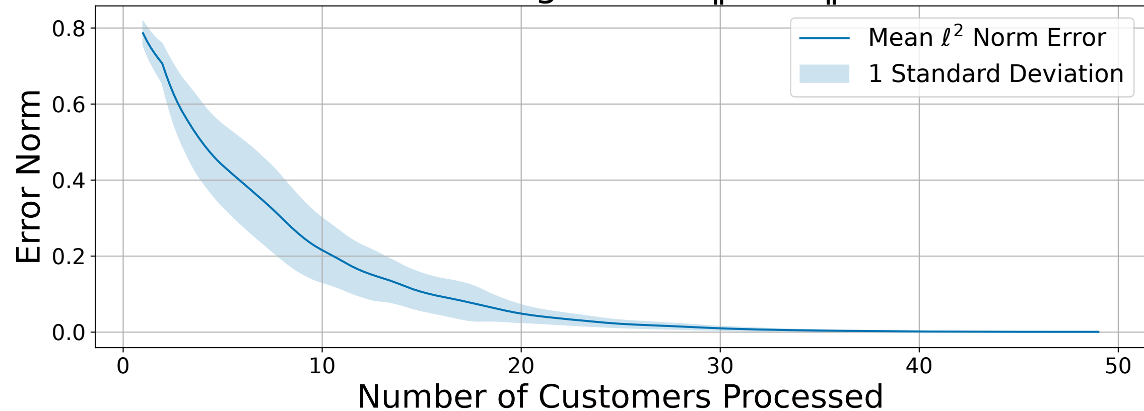
Convergence of \|\hat{u} - u\|
