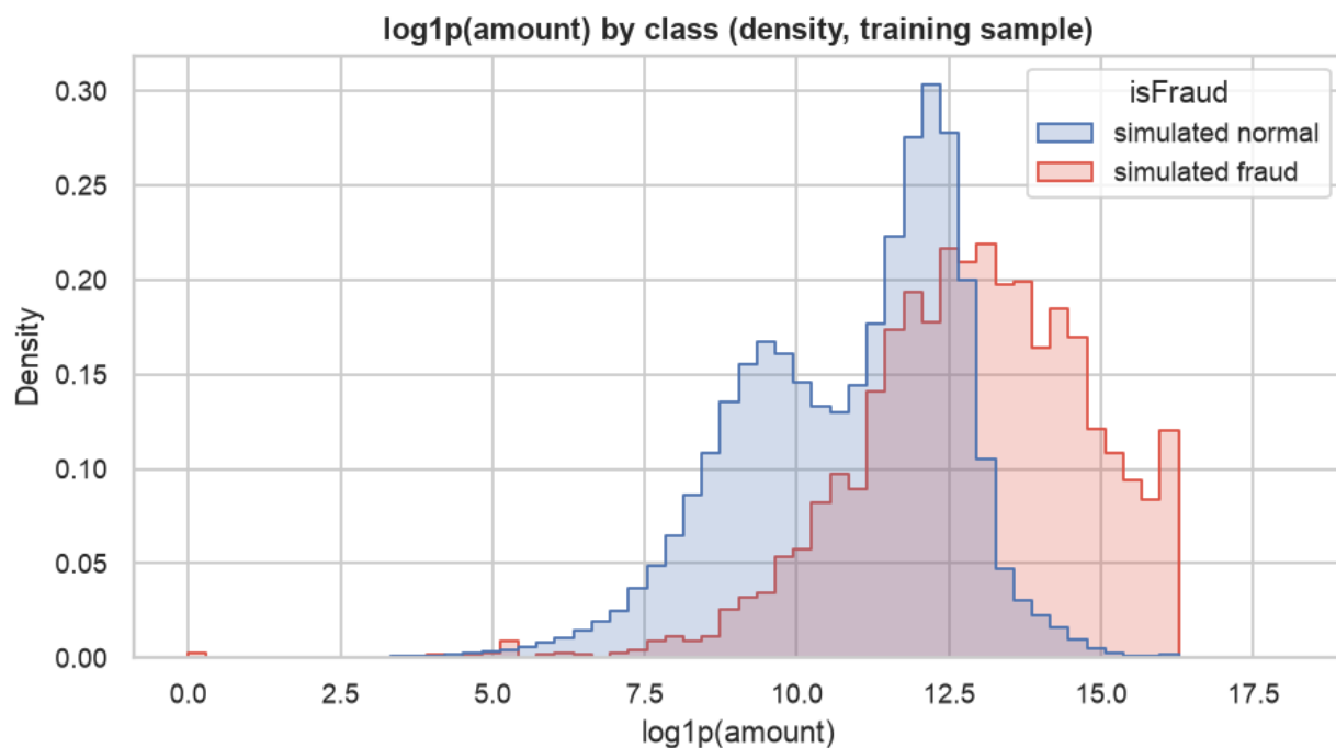
Figure: eda_02_amount_by_class.png
