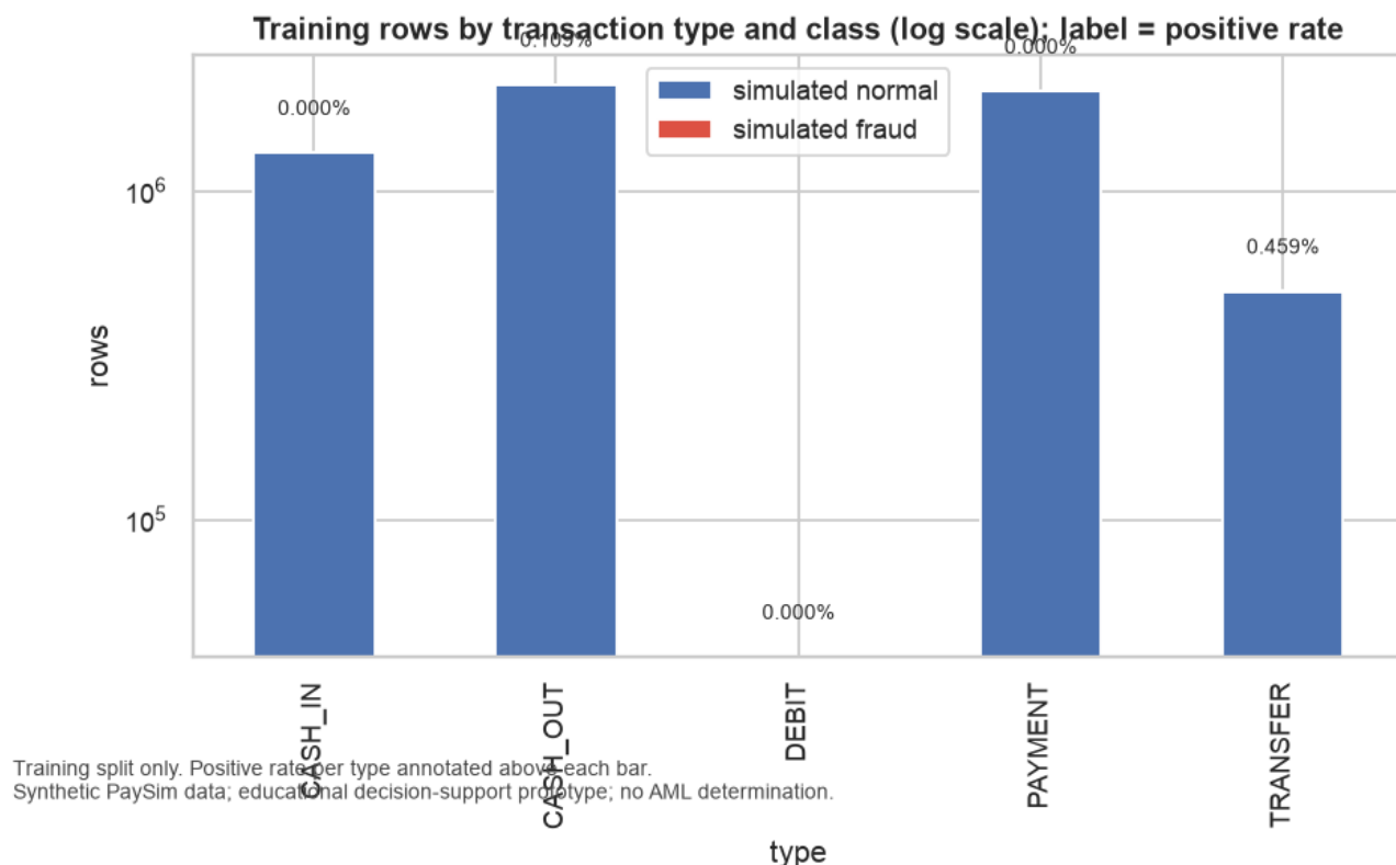
Figure: eda_01_class_by_type.png
