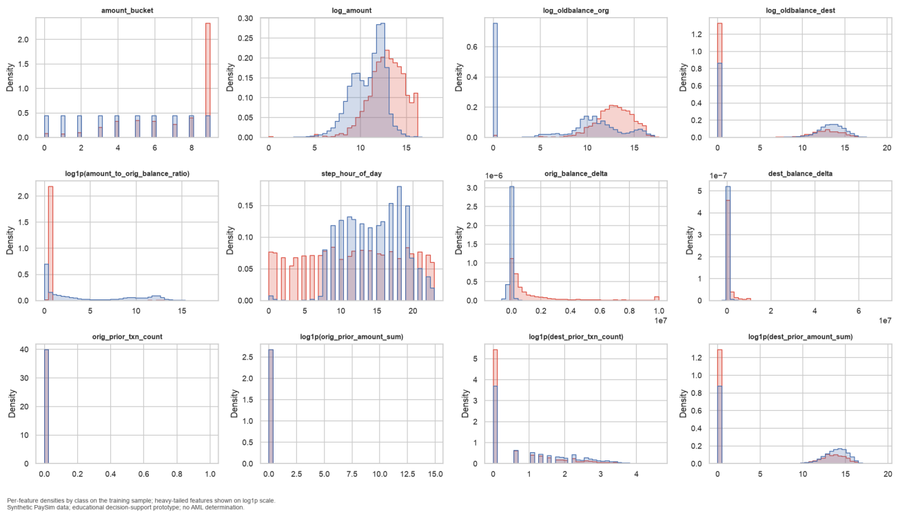
Figure: eda_07_feature_distributions.png
