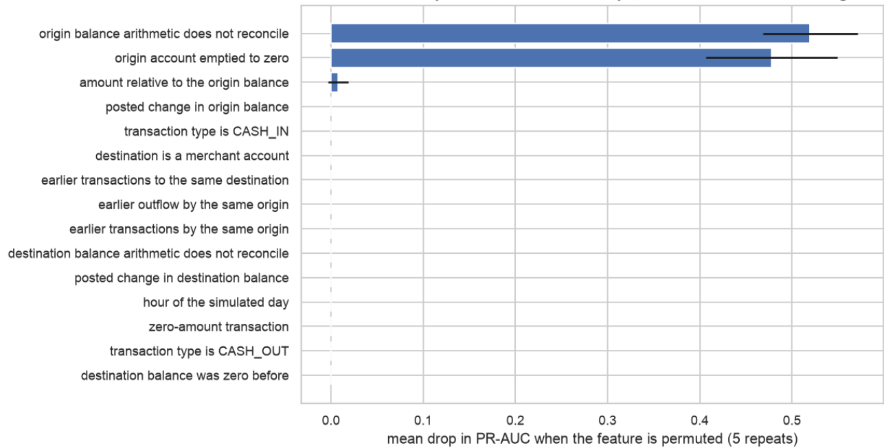
Permutation importance, seeded test sample, 20260904T225142-0dc8f82-hgb
