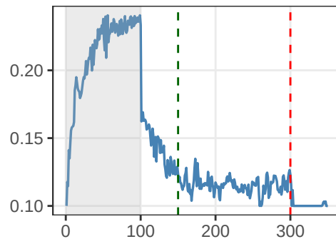
\omega_V
