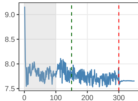
\omega_V
