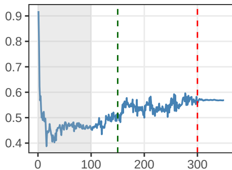
\omega_{k_a}
