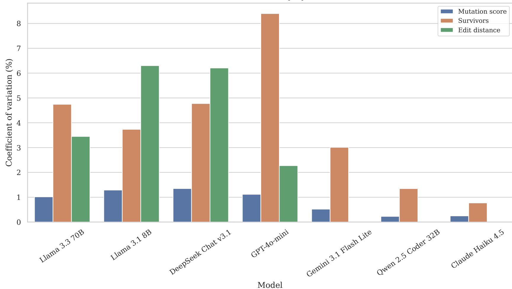
Cross-run variability by metric
