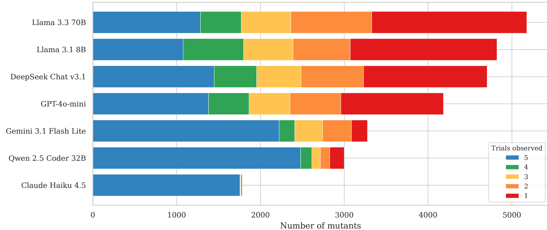
Variability of mutants across runs
