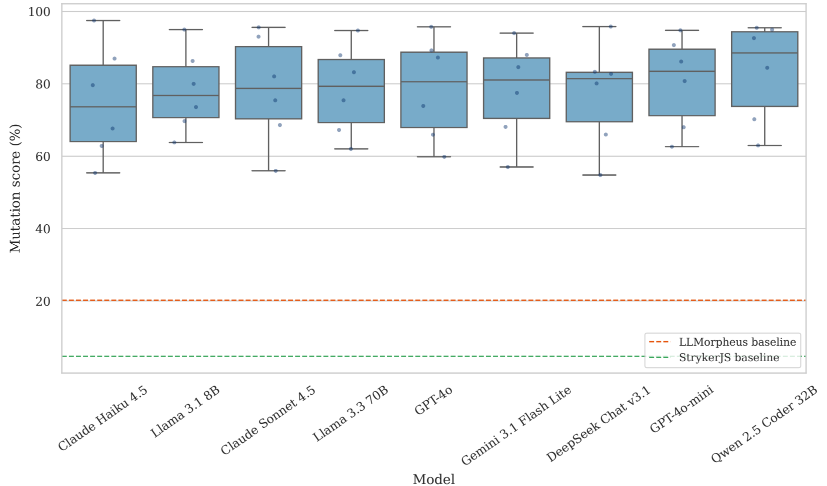
Distribution of mutation scores across packages and runs
