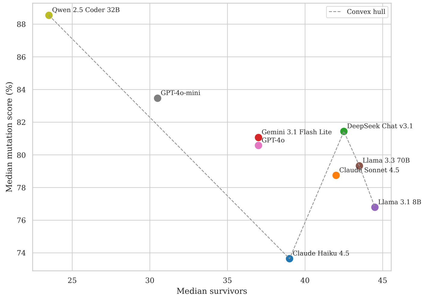
Mutation score vs survivor count
