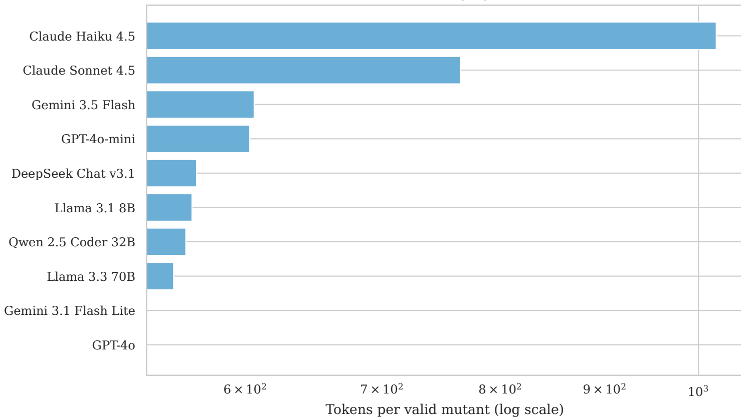
Token efficiency by model
