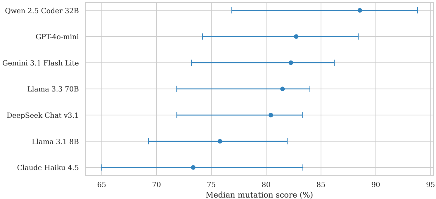
Mutation score with 95% bootstrap CI
