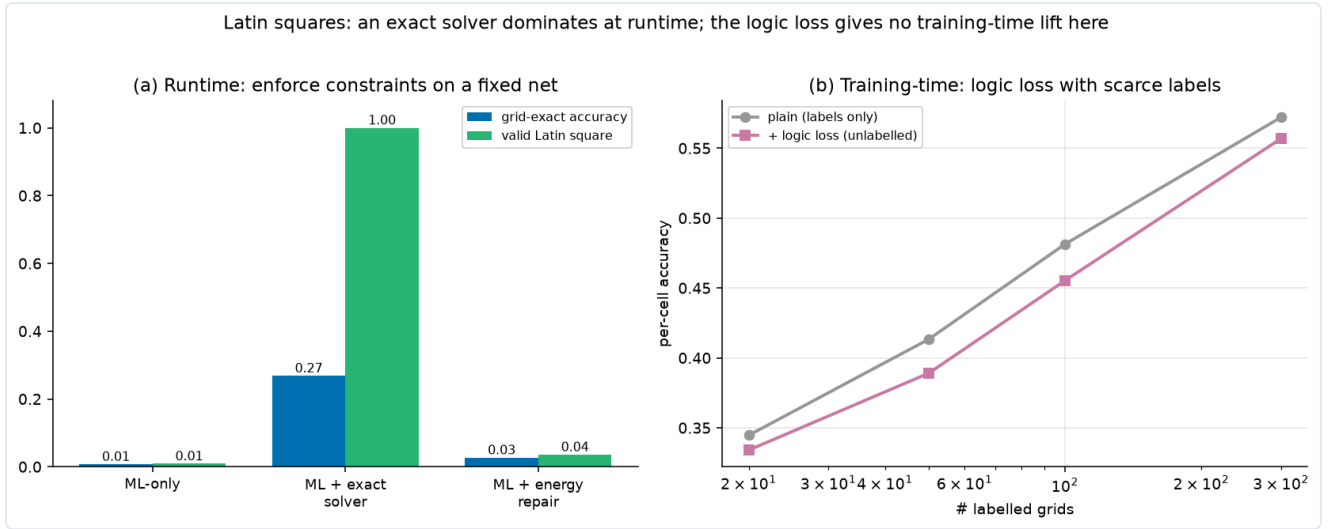
Figure 9. The honest external head-to-head on Latin squares. (a) At runtime an exact solver dominates soft energy repair; (b) at training time the logic loss gives no lift on this permutation-symmetric task. The method wins when you need a gradient, scale past enumeration, or scarce-label target signal — not here.
