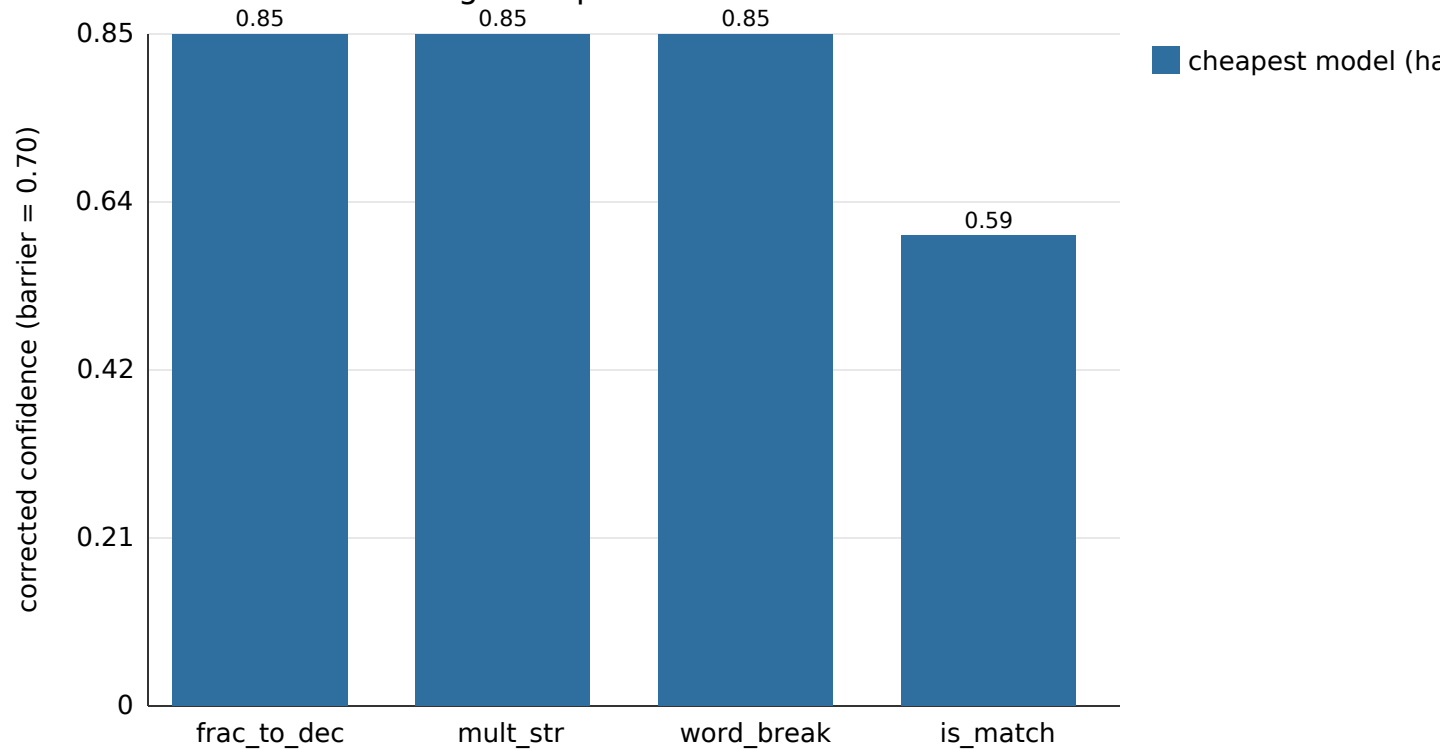
Live broker routing: cheap model's corrected bid vs the 0.70 barrier
