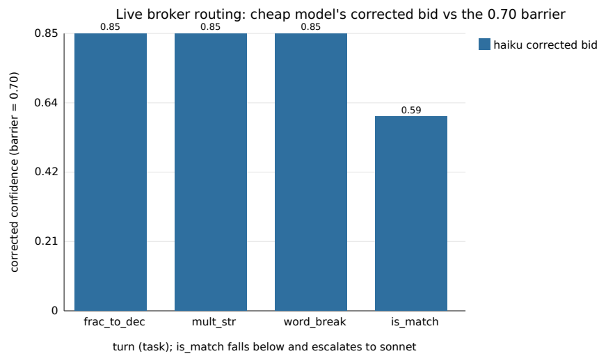
Figure 9: The cheap model's (Haiku) reliability-corrected bid across the four live turns. It clears the 0.70 barrier on the first three tasks, which route to Haiku, and dips to 0.595 on is_match , which escalates to Sonnet.
