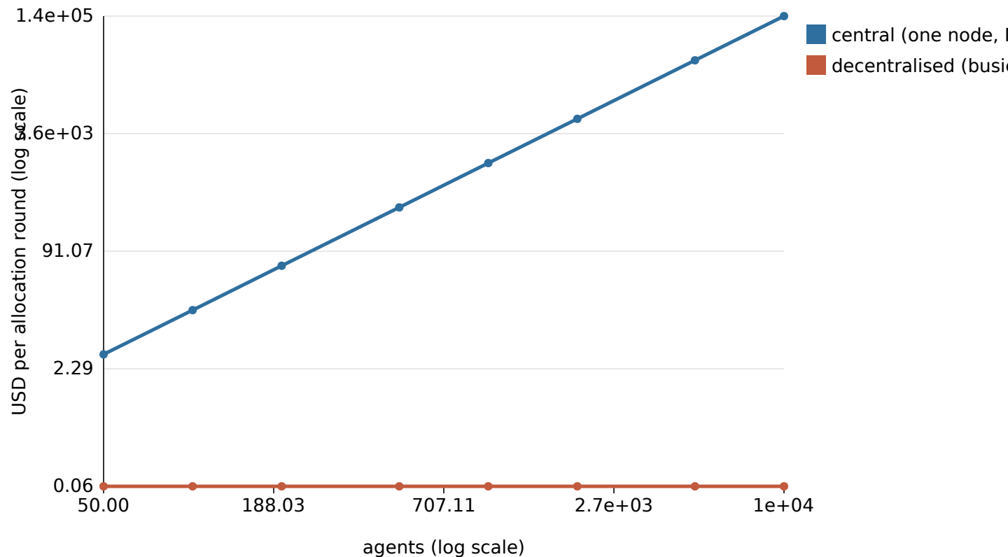
Coordination dollar cost vs agent count (standard tier)
