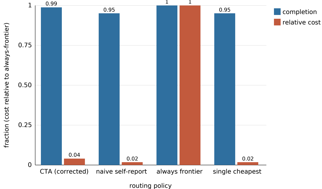
Head-to-head on real agents: completion vs cost by routing policy
