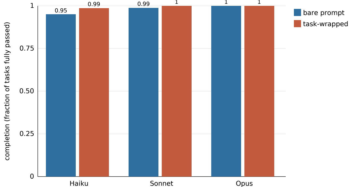
Capability ladder: task completion by model and wrapper
