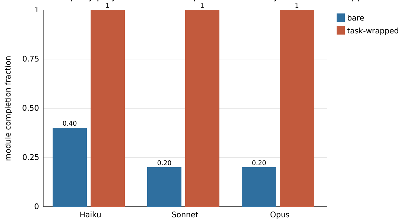
miniquery project: module completion fraction by model and wrapper
