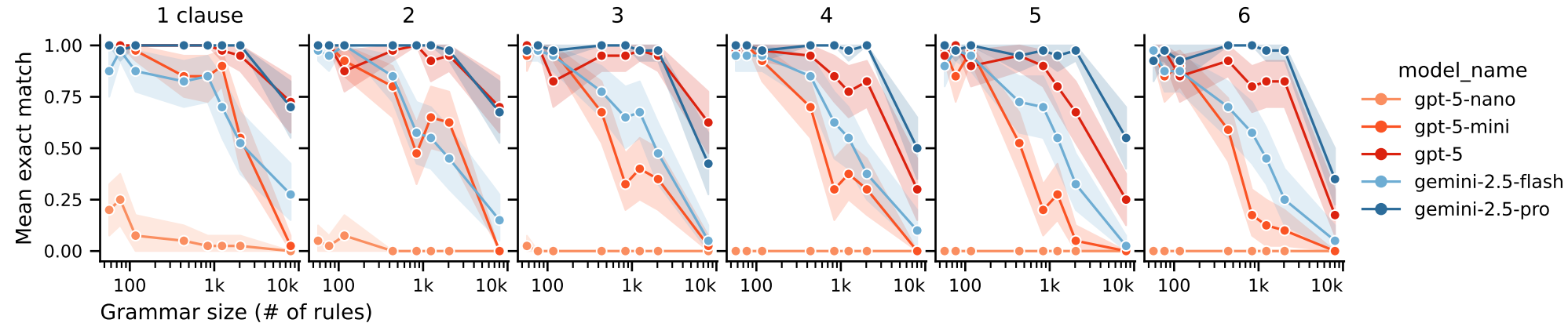
Exact-match accuracy, facted by sentential complexity
