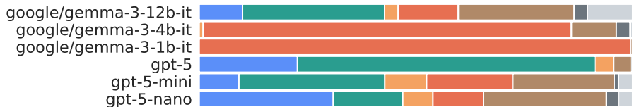
Morphology
