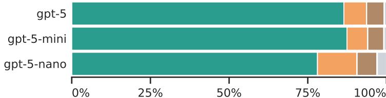
Morphology
