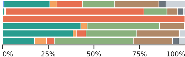
Orthography
