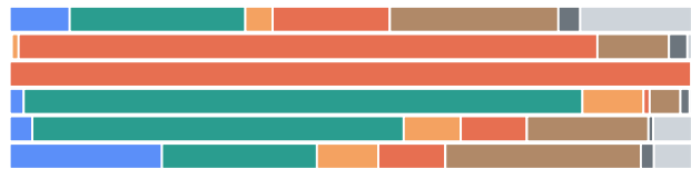
Orthography
