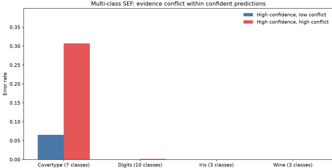
Figure 11: Multi-class evidence conflict inside predictions that already look confident. Covertypes gives the clearest nontrivial test because the confident subset still contains enough errors to compare.
