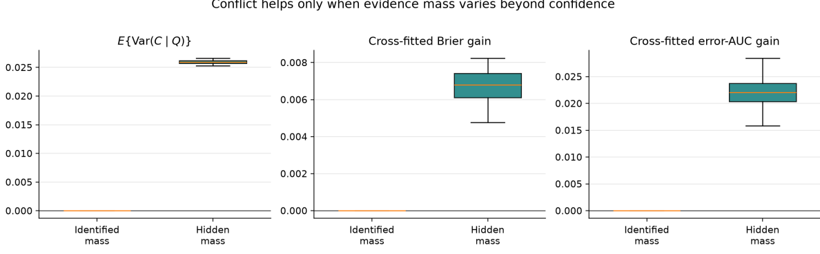
Figure 1: Stress test of the identification boundary. When evidence mass is determined by confidence, conditional conflict variance is zero and adding conflict gives essentially no cross-fitted Brier or error-AUC gain. When evidence mass varies within confidence levels and loss changes with conflict, both gains become positive.
