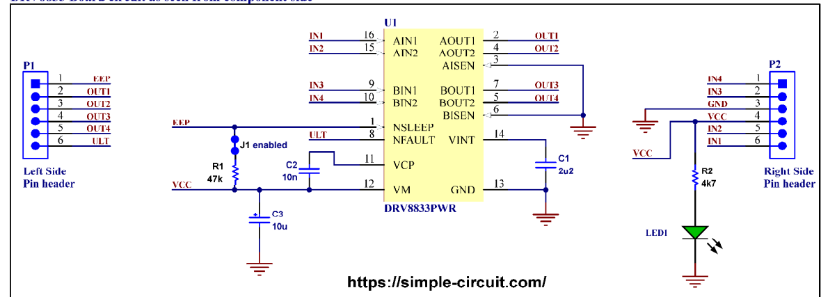
DRV8833 Board circuit as seen from component side
