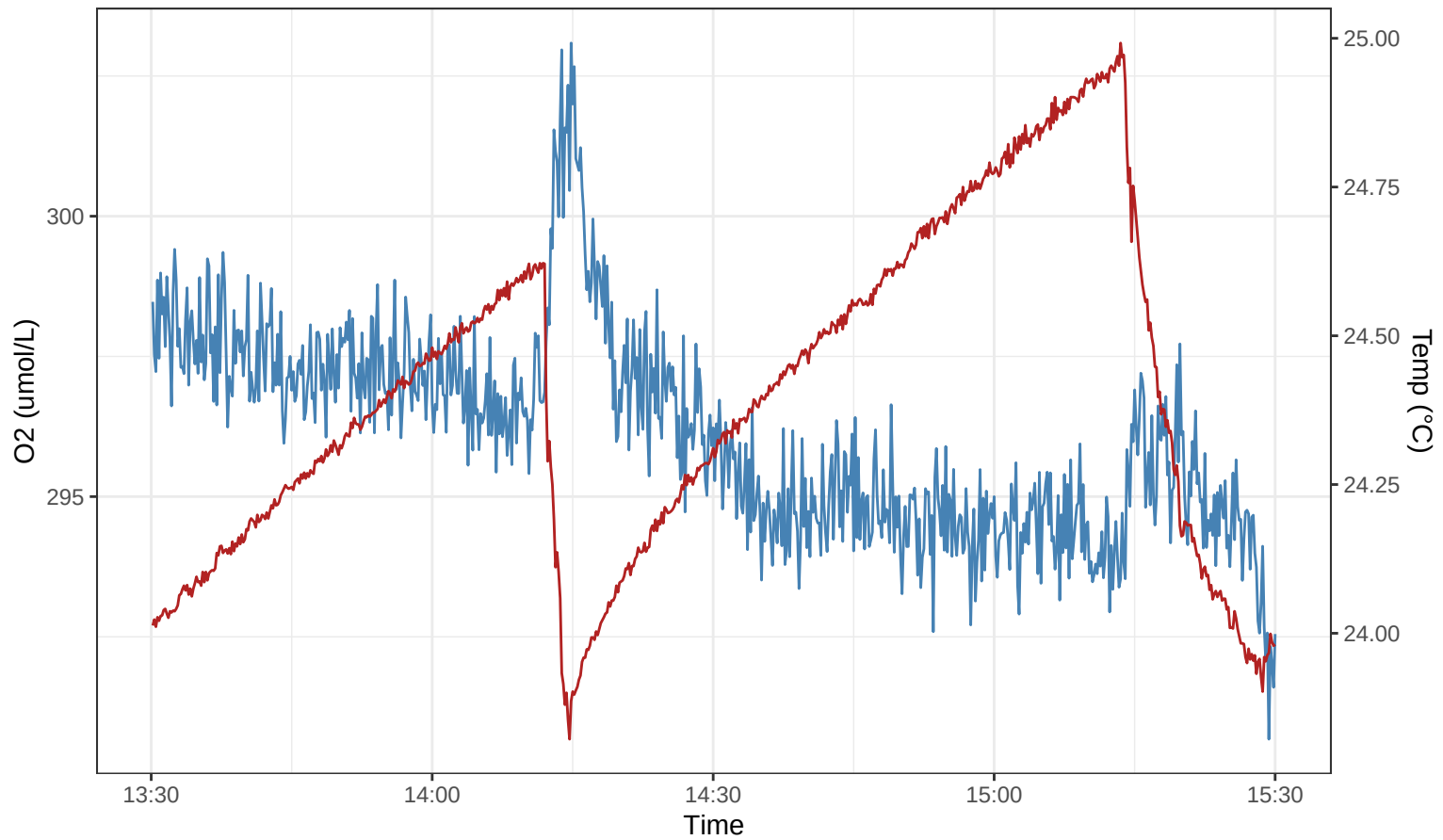
S2.4_RUN4 – O2 (blue) vs Temp (red)
