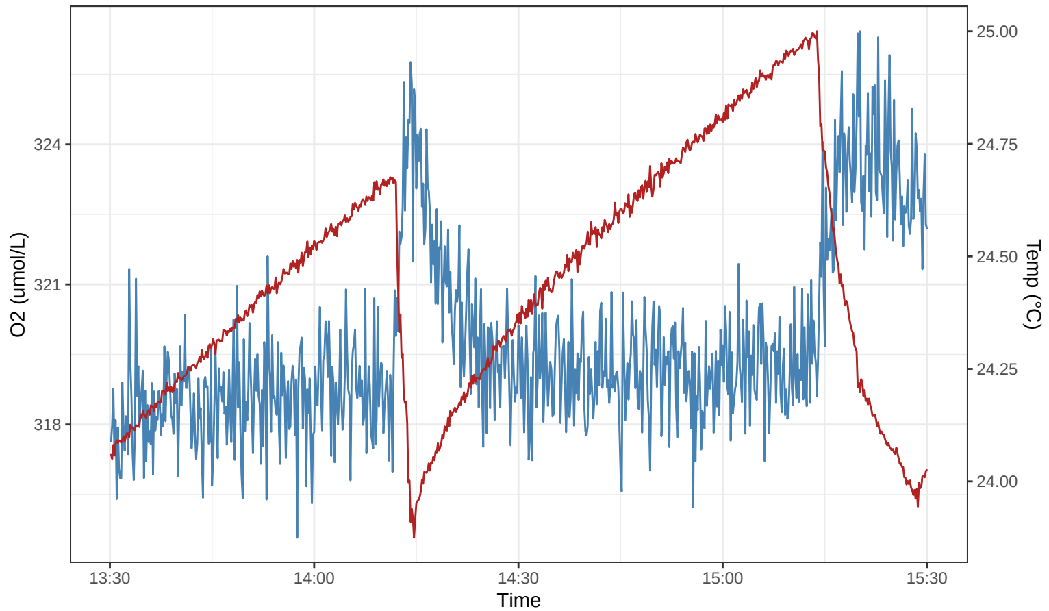
S1.1_RUN4 – O2 (blue) vs Temp (red)
