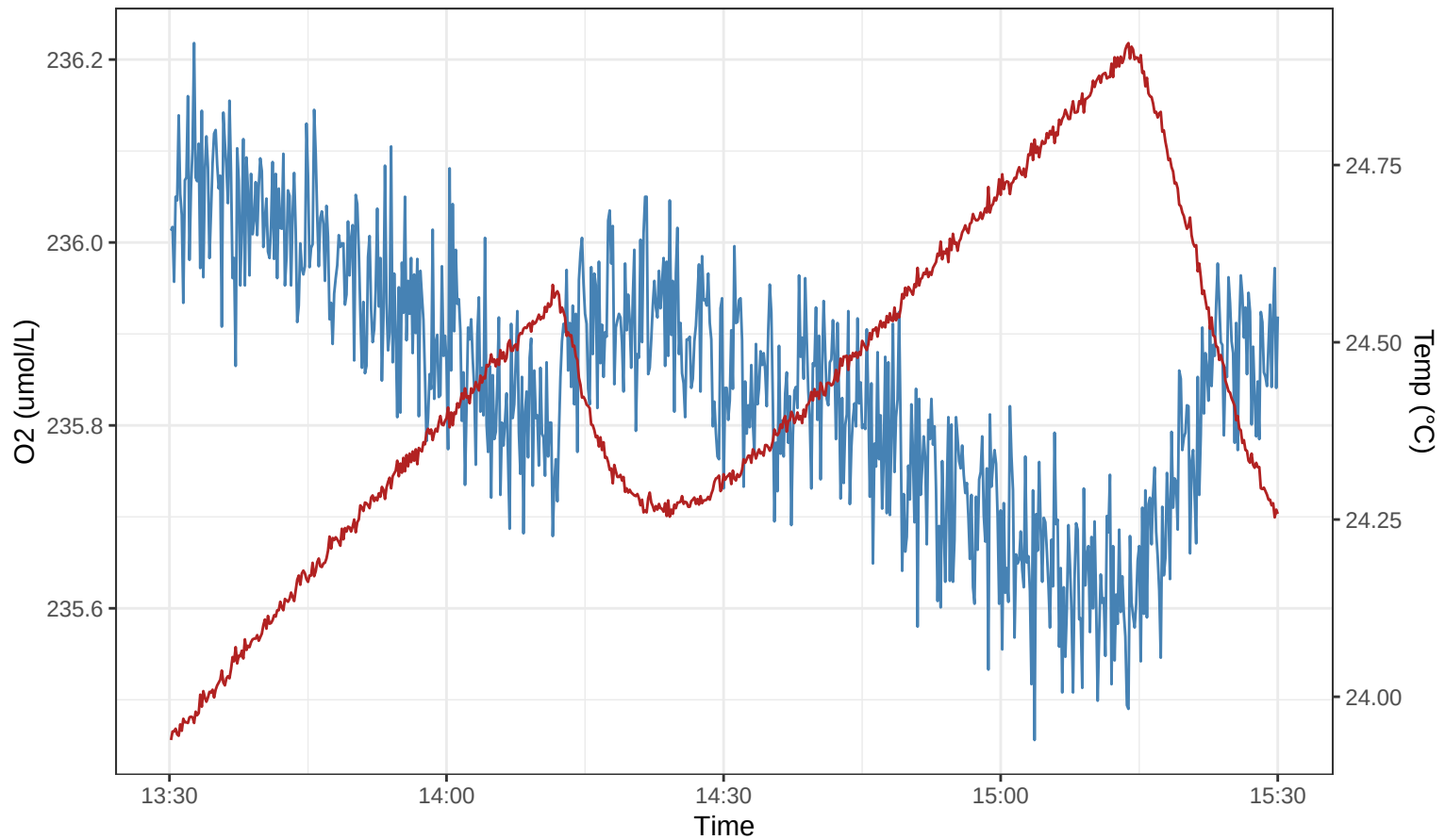
S2.2_RUN4 – O2 (blue) vs Temp (red)
