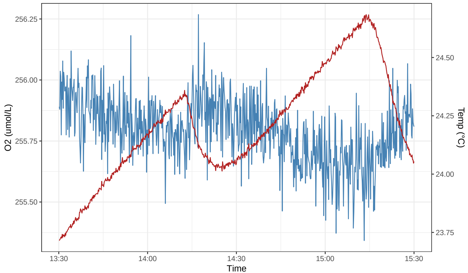
S2.1_RUN4 – O2 (blue) vs Temp (red)
