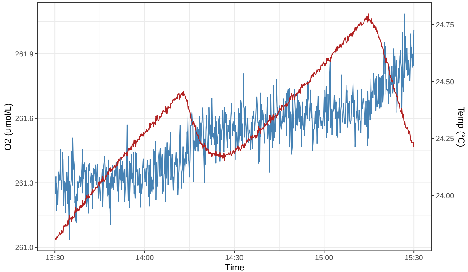
S1.2_RUN4 – O2 (blue) vs Temp (red)
