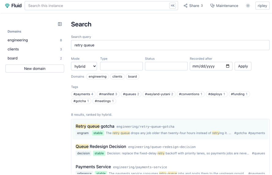
Figure 4.2: Faceted search across the instance, backed by the ranking the agents use.
