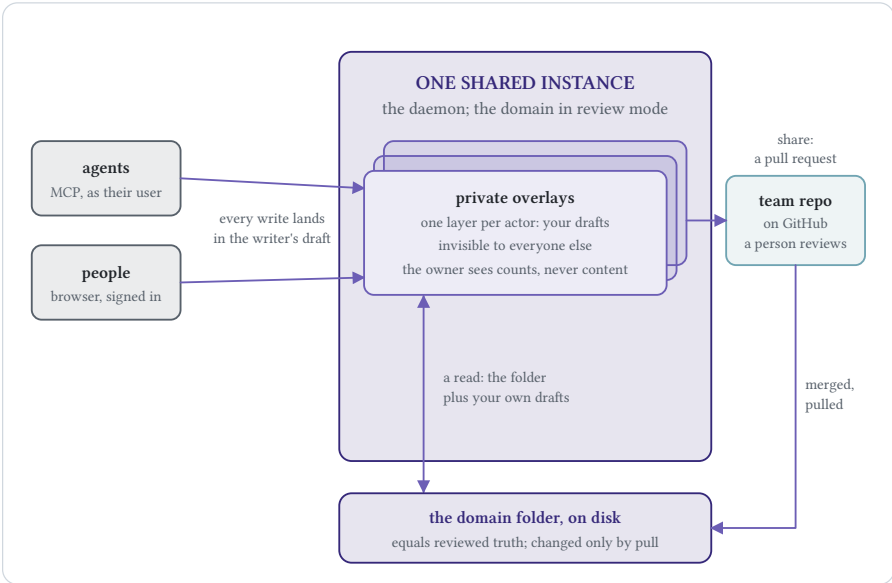
Figure 13.2: One shared instance in review mode: each actor drafts in a private overlay above the domain folder, a draft goes out as a pull request, and only a merged pull changes the folder.
