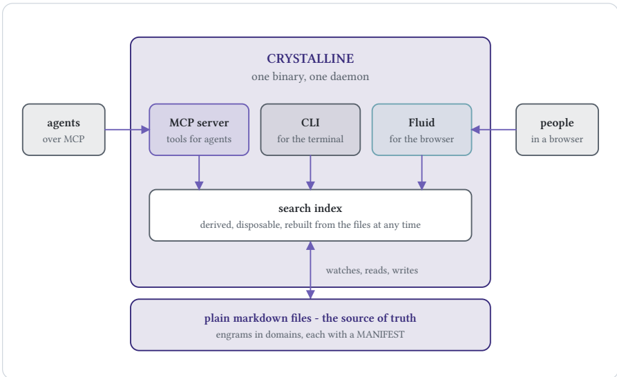
Figure 4.1: One binary: the CLI, the MCP server, Fluid and the search index, all standing on plain markdown files. Agents come in through MCP, people through Fluid.
