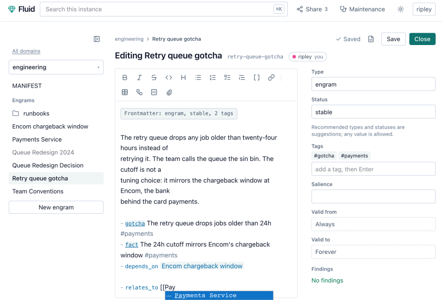
Figure 9.1: Editing an engram in Fluid: live preview, the frontmatter form and wikilink completion.
