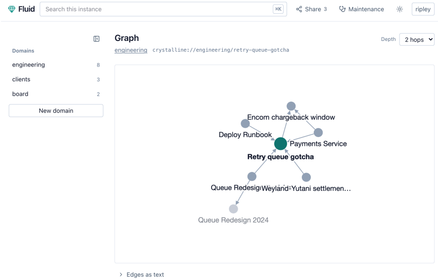
Figure 4.3: The neighbourhood graph of an engram in Fluid.
