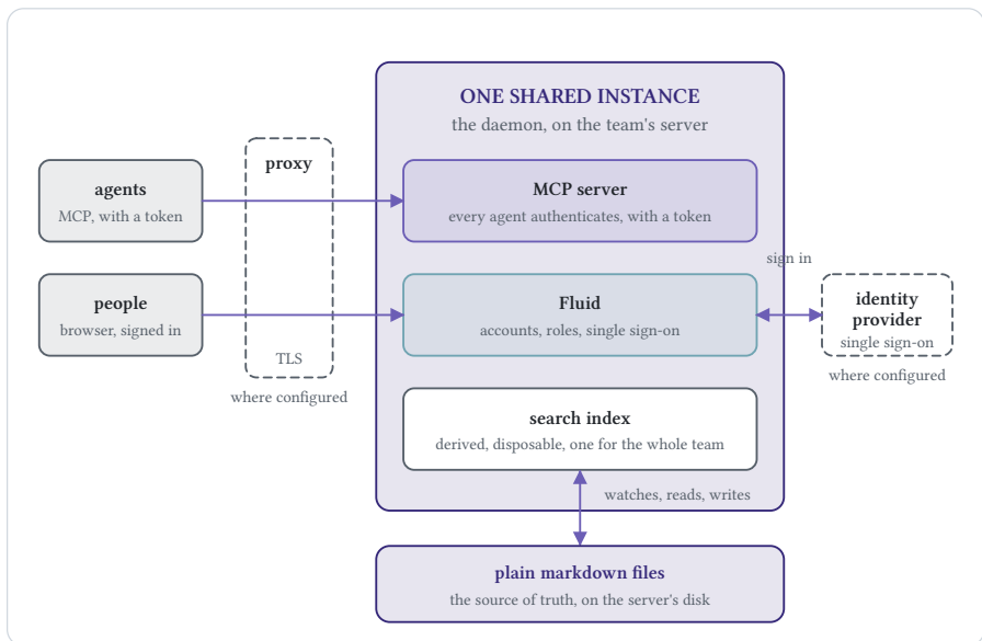
Figure 7.1: One shared instance: agents connect over MCP with a token, people through Fluid with an account, with a proxy in front and an identity provider beside it where the team configures them.
