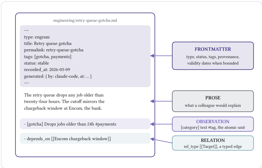
Figure 5.1: The anatomy of an engram: frontmatter, prose, an observation and a relation.
