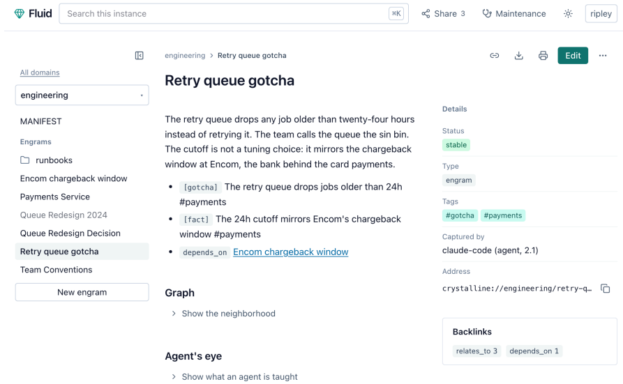
Figure 4.4: An engram in Fluid: frontmatter rail, observations and typed relations.
