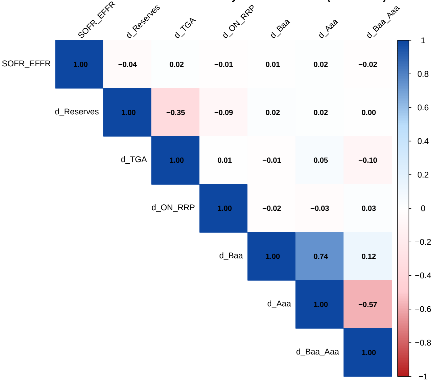
Correlation Matrix: Stationary Transformations (Post-2018)
