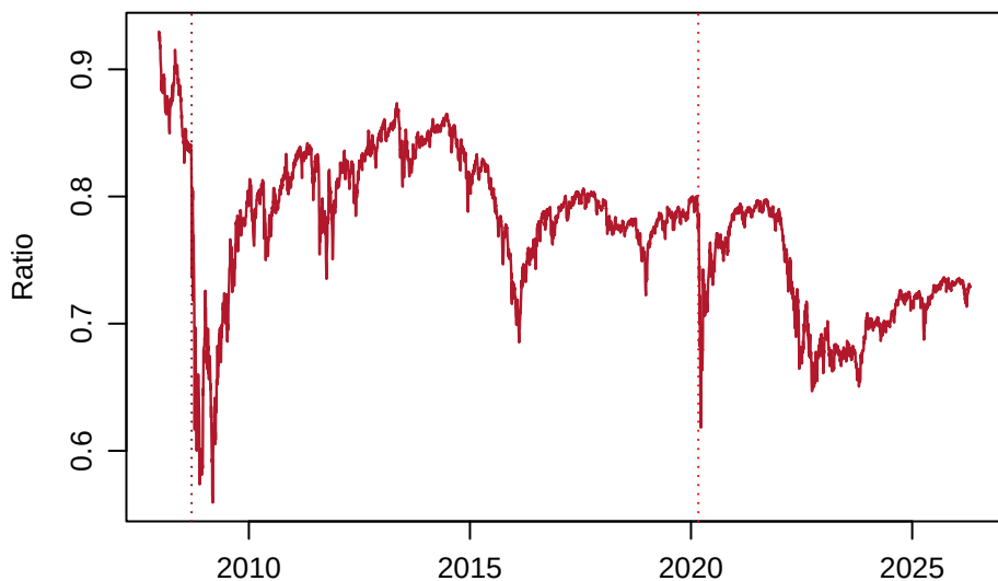
(c) HYG/SHV (Flight to Quality)
