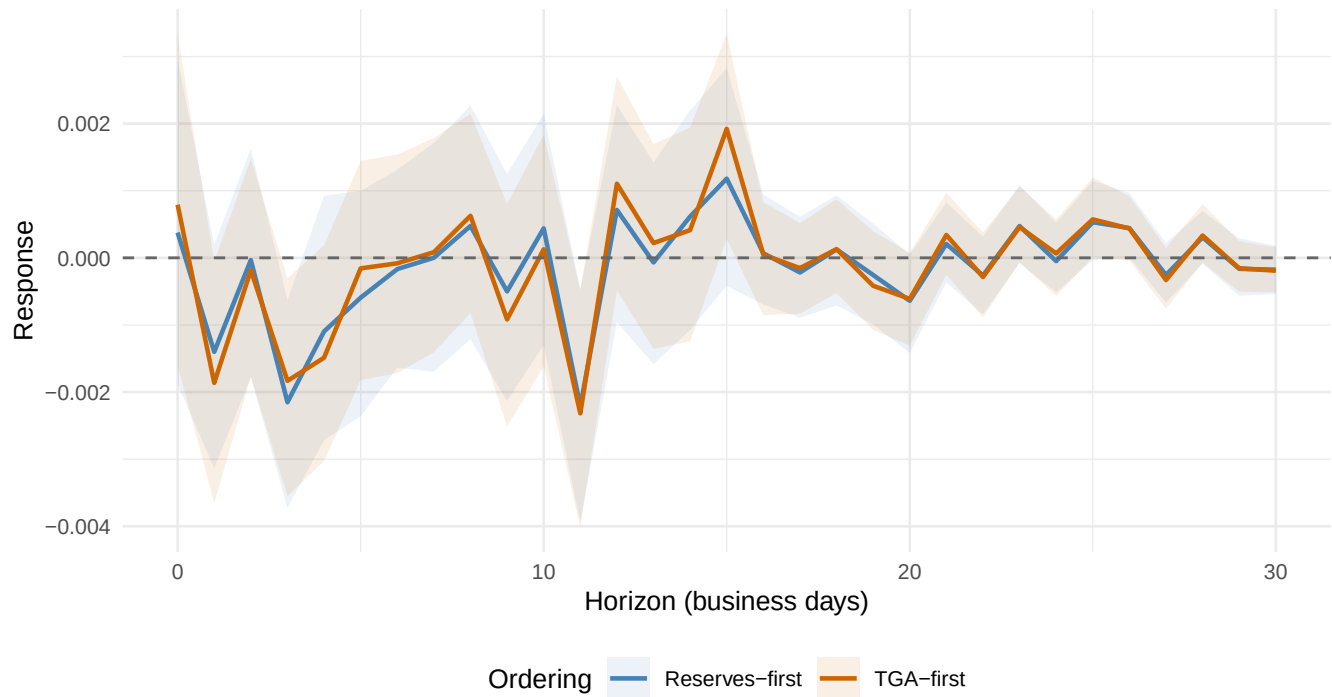
Robustness: Response of d_Aaa to d_Reserves shock under alternative Cholesky orderings
