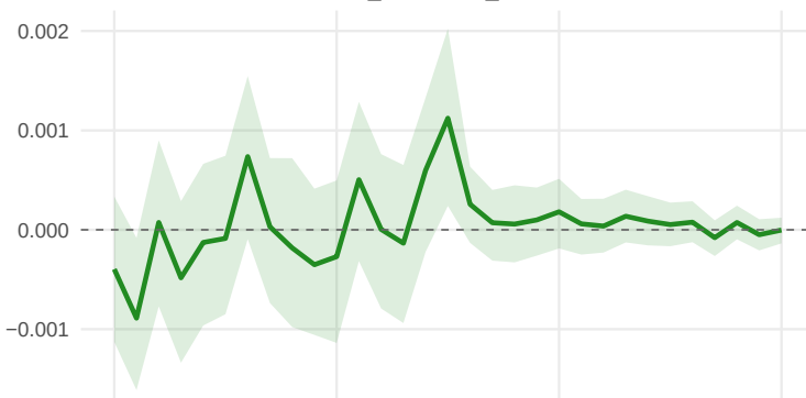
d_TGA -> d_Baa
