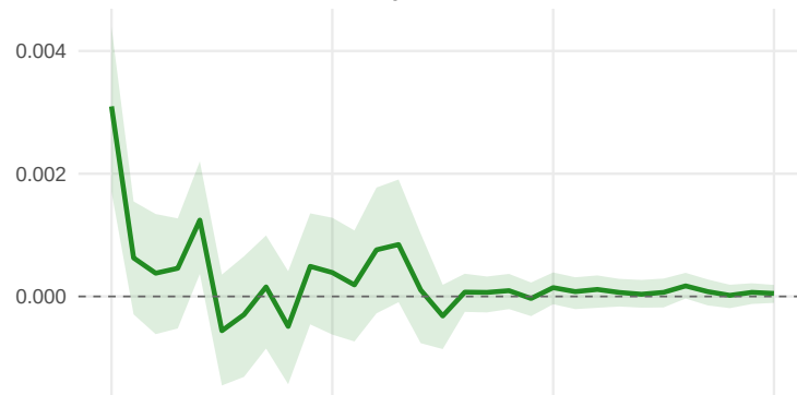
d_Reserves -> d_Aaa
