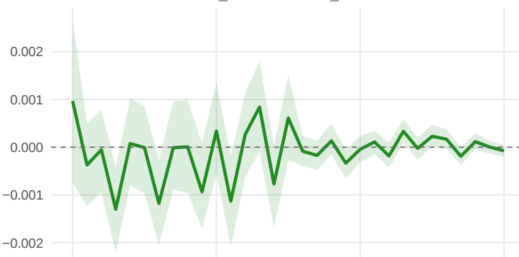
d_TGA -> d_Aaa
