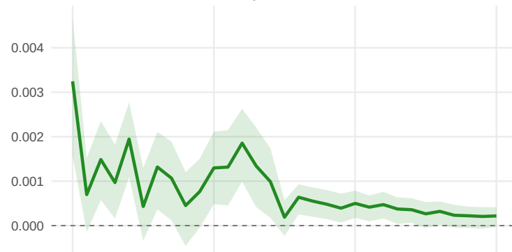
d_Reserves -> d_Baa
