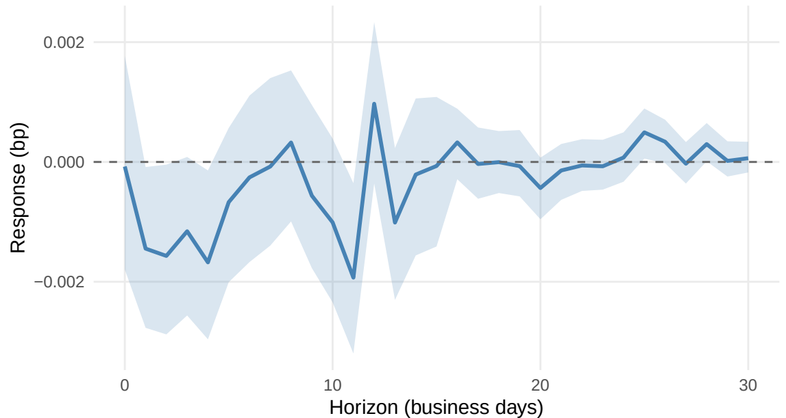
Response of d_Baa to d_Reserves shock (Cholesky, Post-2018)
