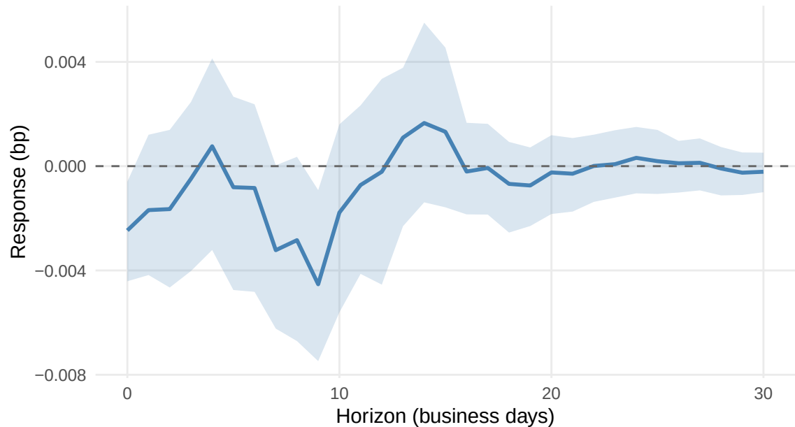
Response of SOFR-EFFR to d_Reserves shock (Cholesky, Post-2018)
