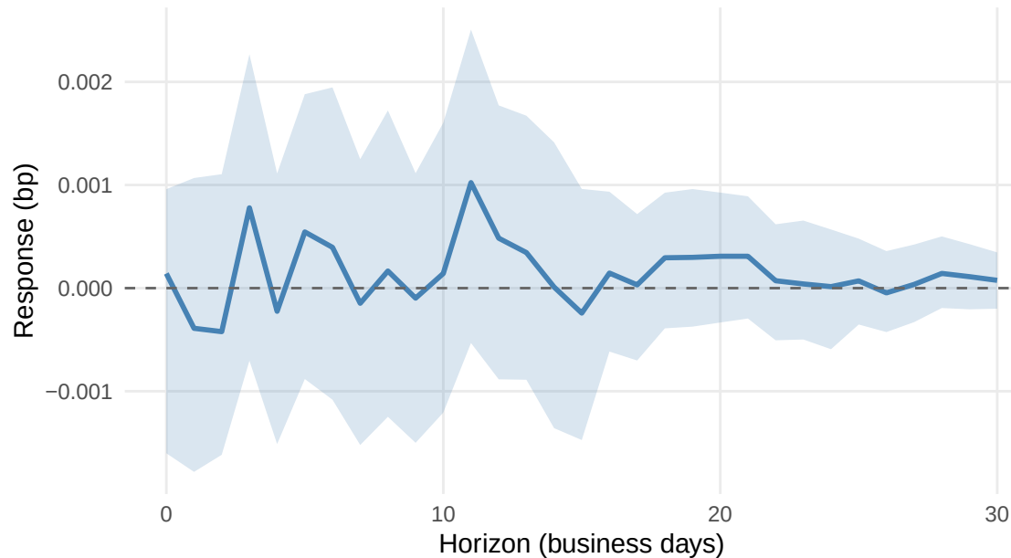
Response of d_Baa to SOFR-EFFR shock (Cholesky, Post-2018)
