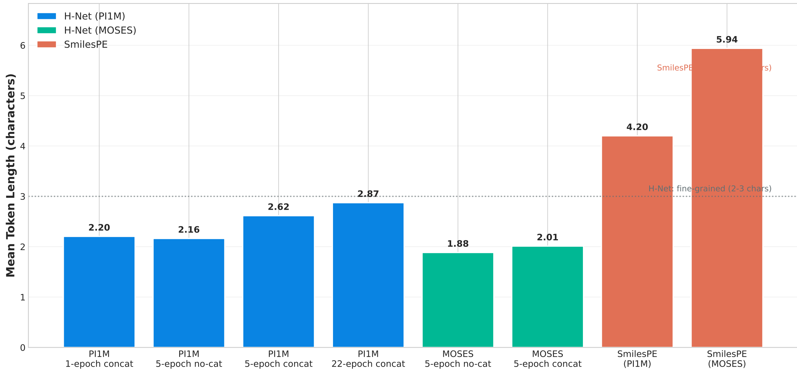
Token Length Comparison: H-Net Models vs SmilesPE
