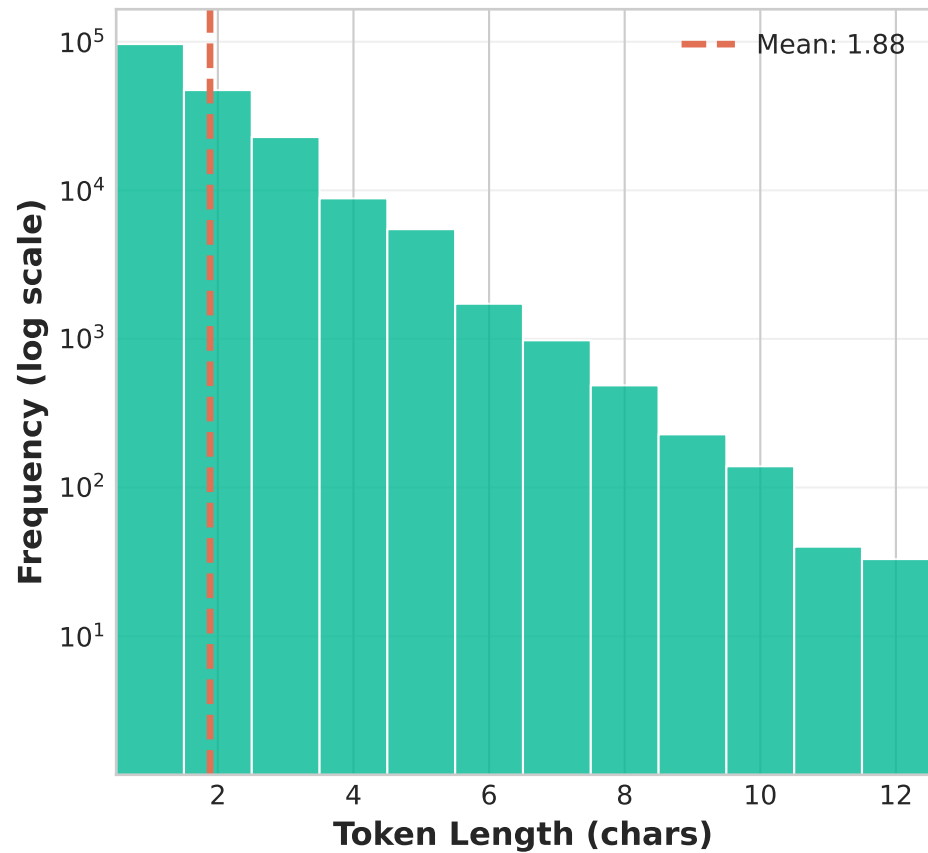
(b) MOSES (Molecular)
