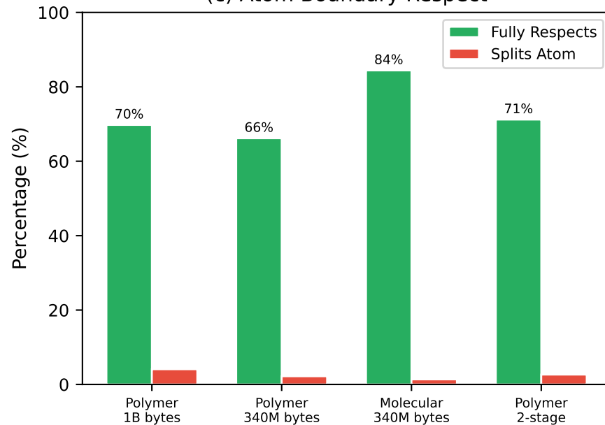
(c) Atom Boundary Respect
