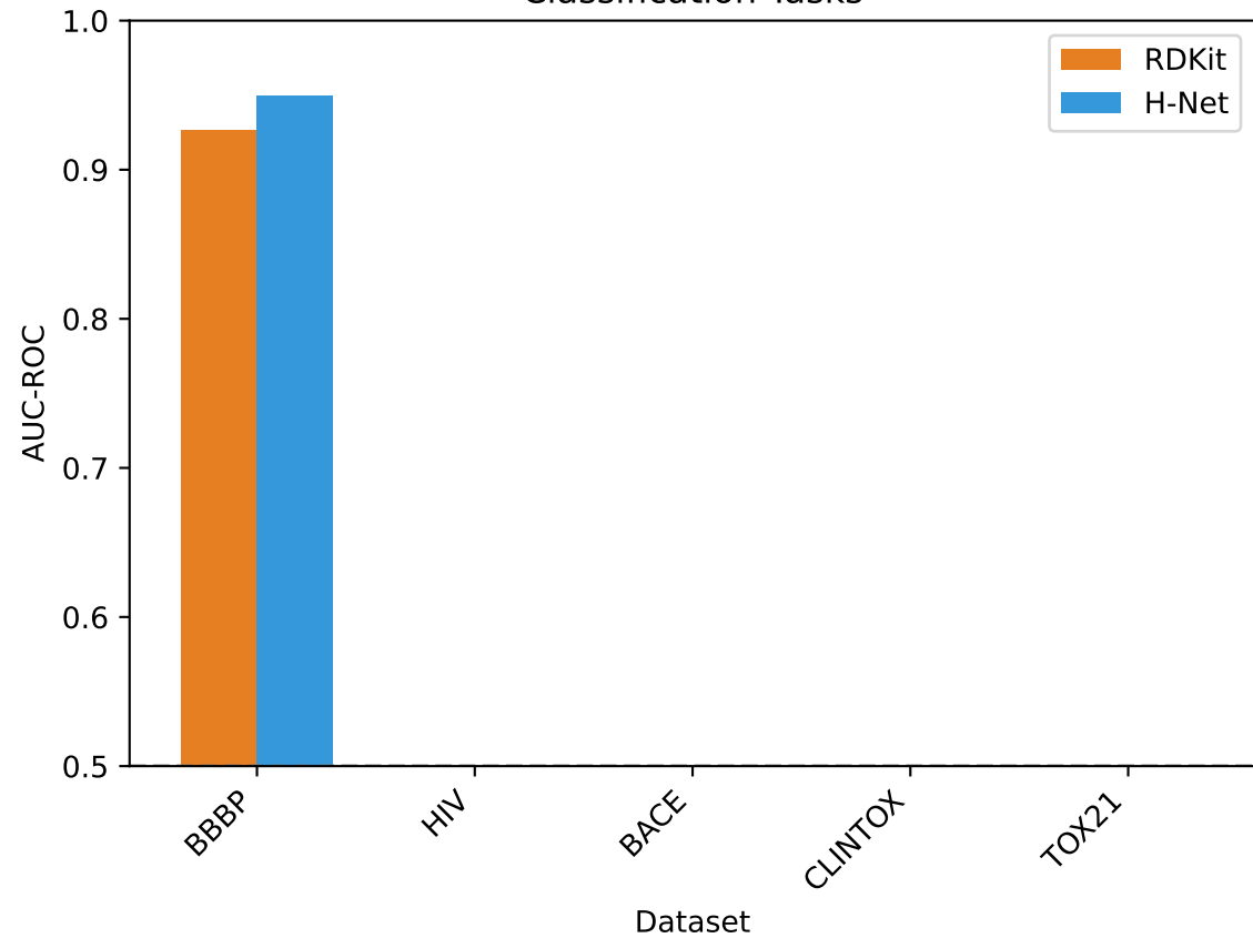
Classification Tasks
