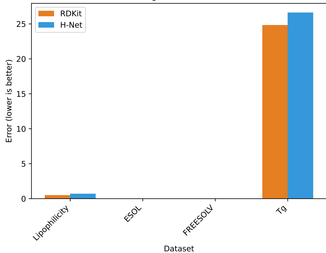
Regression Tasks
