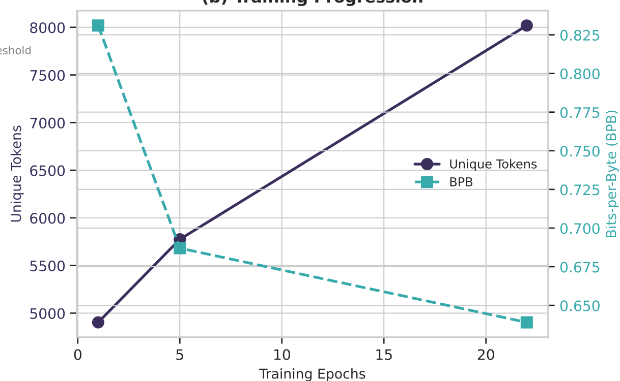
(b) Training Progression
