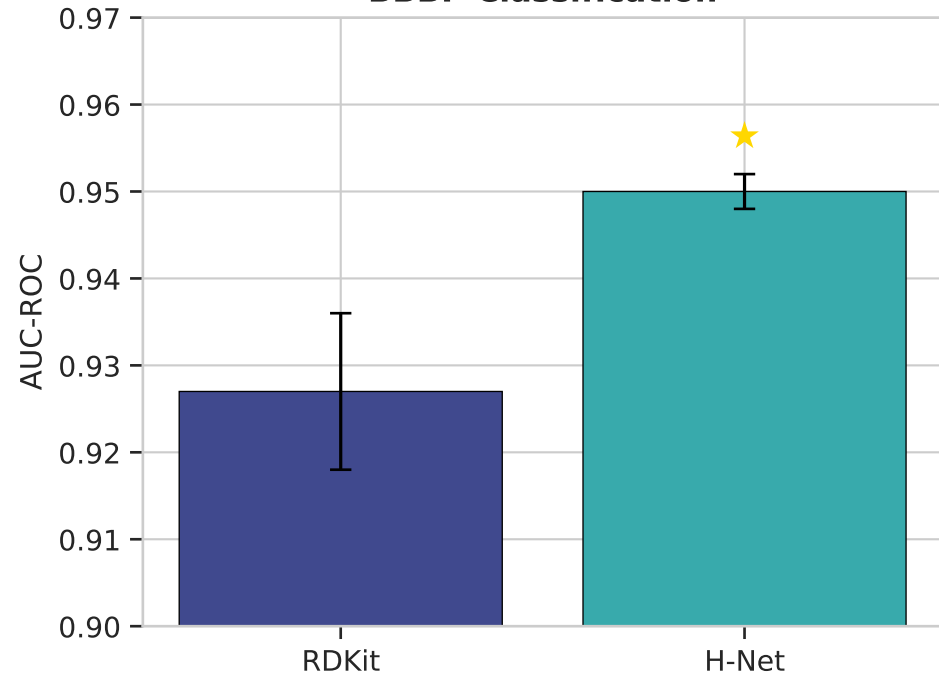
BBBP Classification
