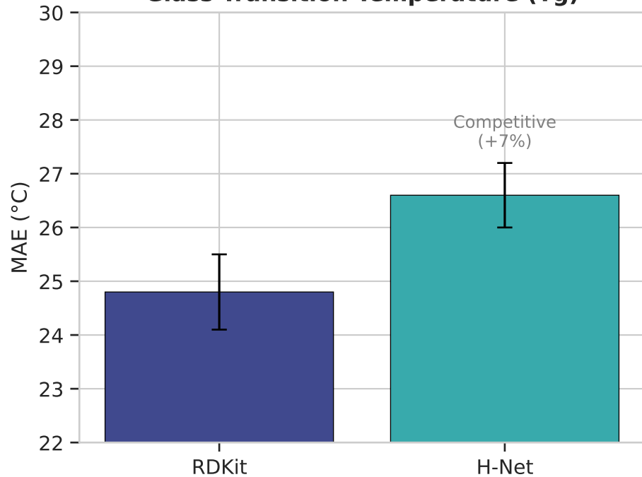
Glass Transition Temperature (T g )
