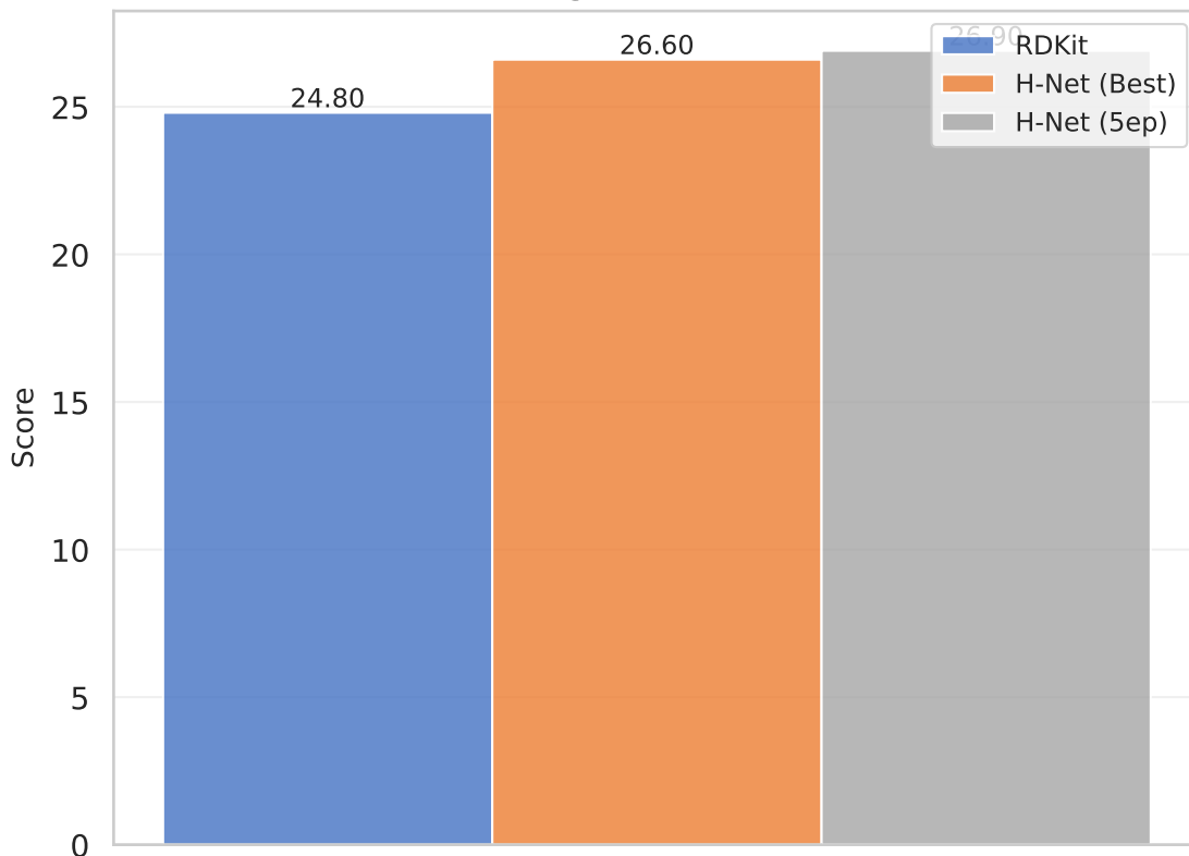
Lipophilicity (MAE)
