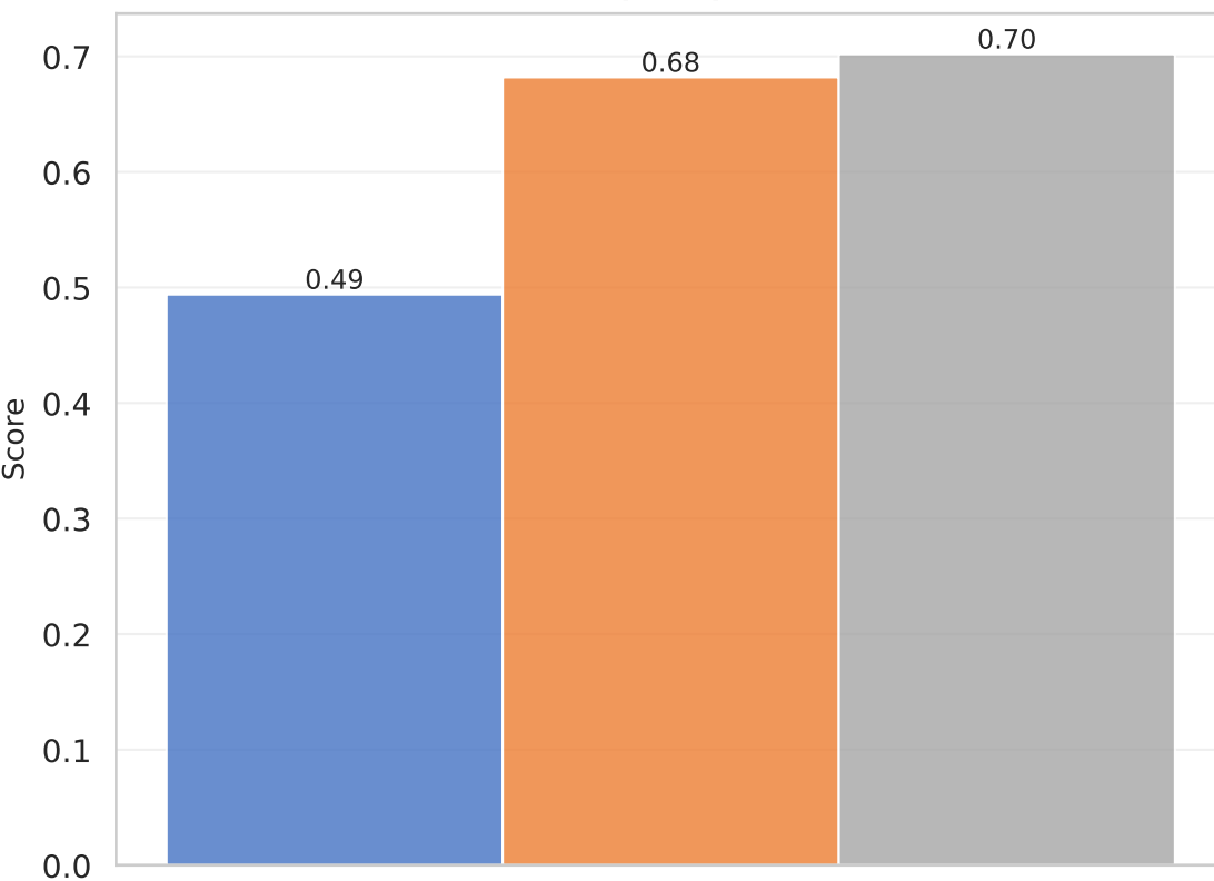
Lipophilicity (MAE)
